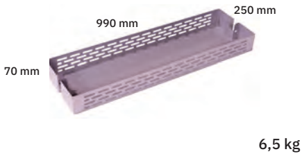
VERKTYGSTAVA / TOOL PANEL Article no. 608033 Article no. 608033-269 Article no. 608033-270
