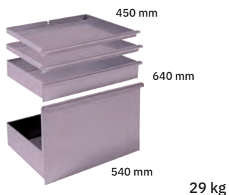
SOPHINK / WASTE BUCKET Article no. 601021
